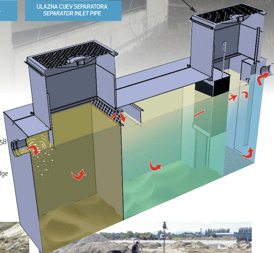
MONTAŽNO KLIZNO GRLO MOUNTABLE SLIDING THROAT
