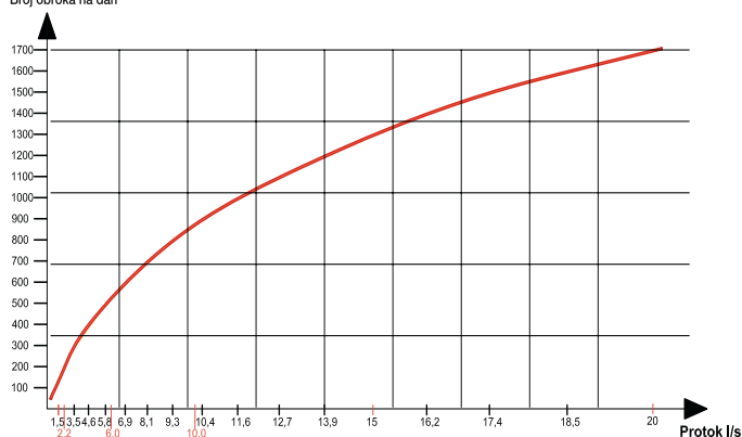
Dijagram protoka mastolova u ovisnosti o broju obroka Graphic outline for determination of grease trap size
